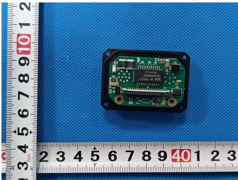
Photo 14: PCB view
