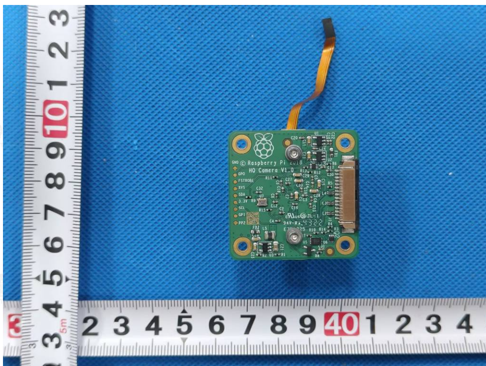
Photo 21: PCB view
