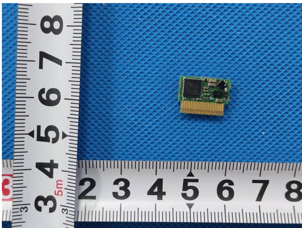
Photo 20: PCB view
