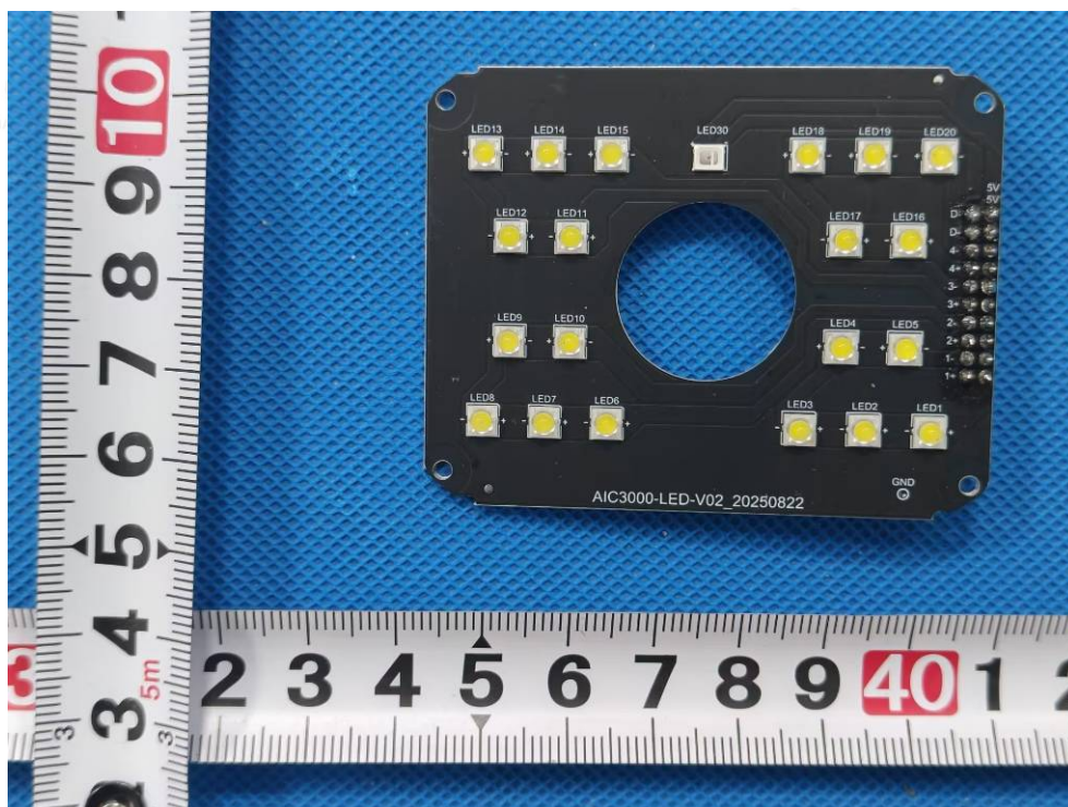
Photo 18: PCB view
