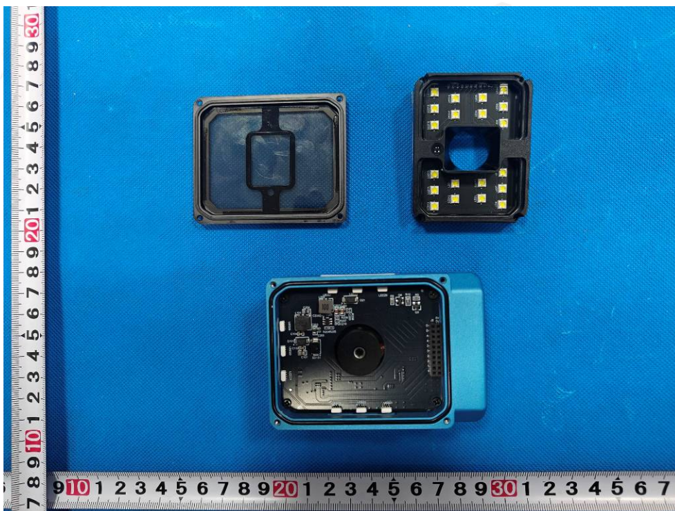
Photo 8: Internal view
